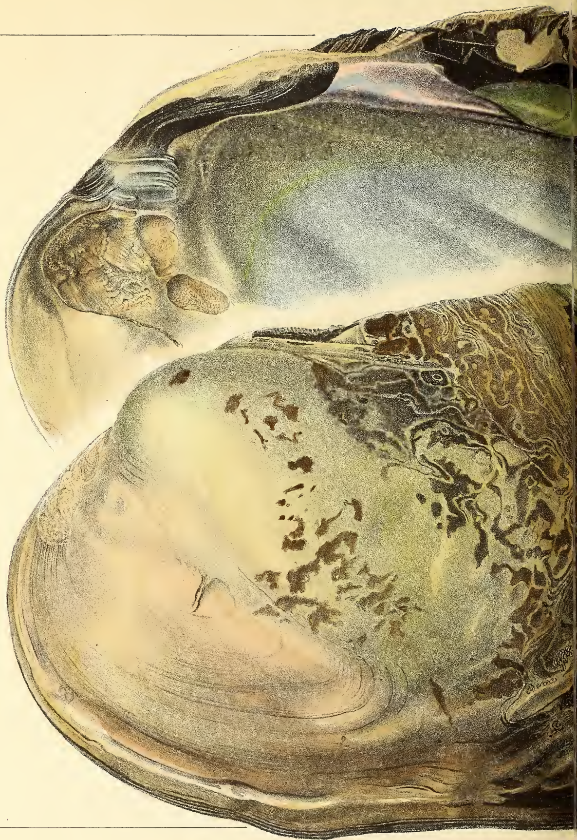
Fig. 1. Chamberlainia hainesia
